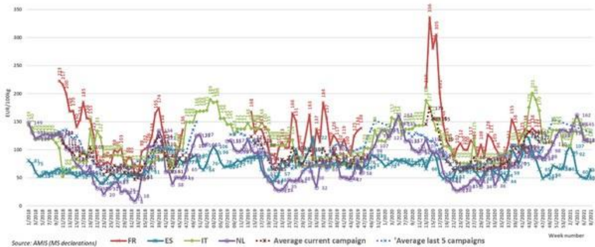
Weekly prices - TOMATOES ESP,IT,NL,FR (main producers of tomatoes)
